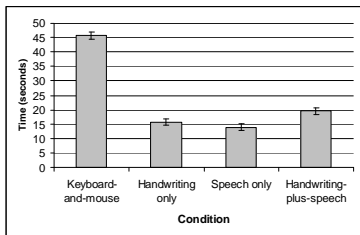
Figure 1. Average time in seconds per equation (from [2]).
