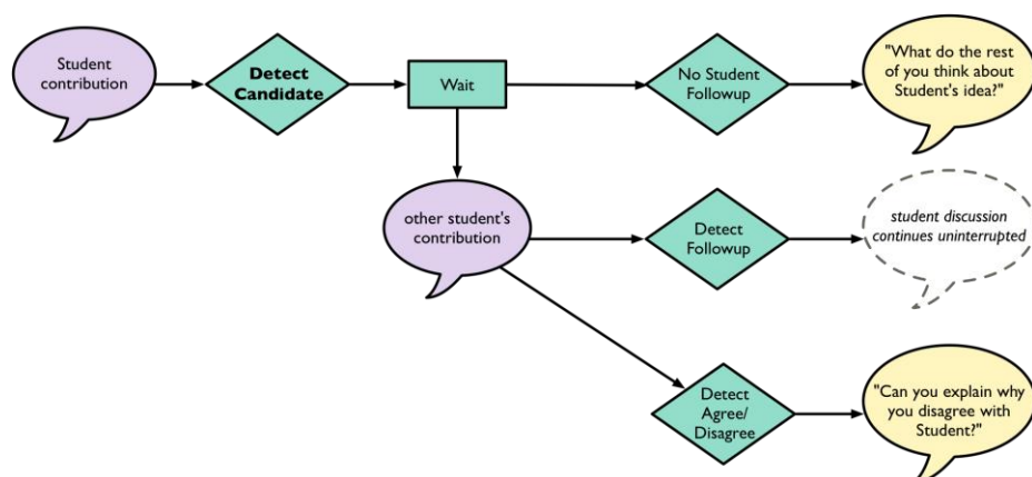
Figure 4. The Agree-Disagree move only triggers in the absence of productive student followup.
