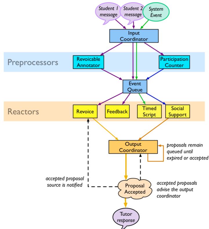
Figure 2. In the Bazaar pipeline, Events are processed in two stages.
