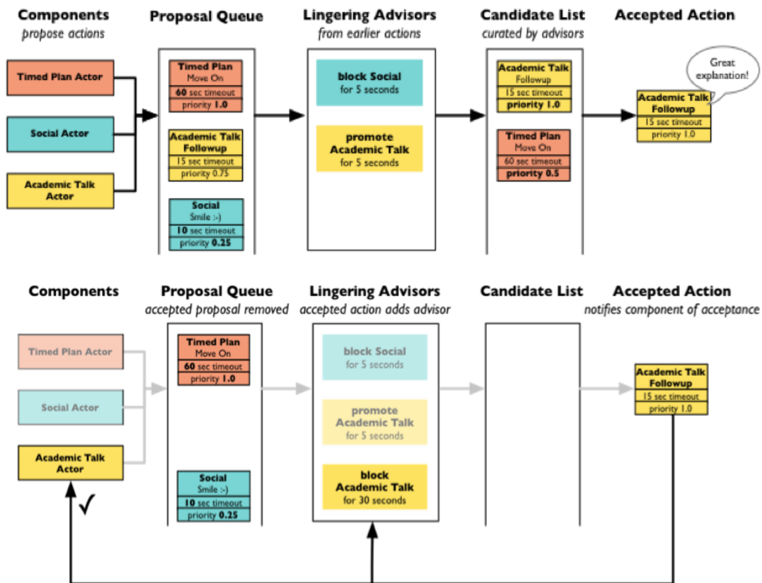
Figure 3. Proposals are managed by the Output Coordinator.
